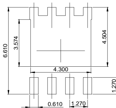
DIMENSIONS: MILLIMETERS
