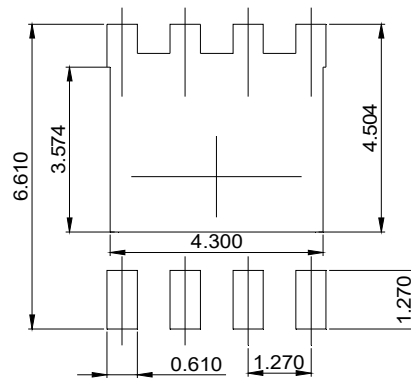
DIMENSIONS: MILLIMETERS
